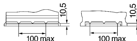
Hold-down
