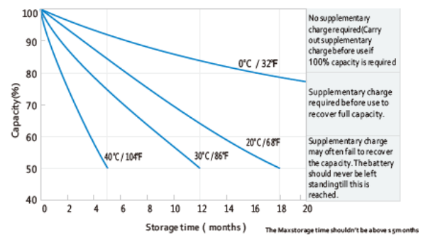
Self-discharge Characteristic
