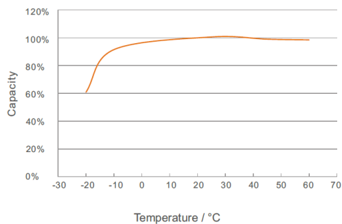
Capacity With Different Temperature
