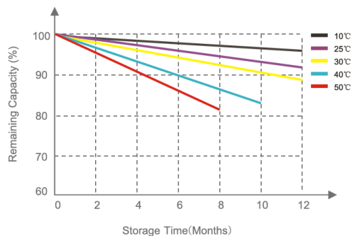
Discharge Capacity At Various Temperatures Discharge @ 1C
