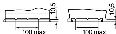
Hold-down
