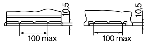
Hold-down
